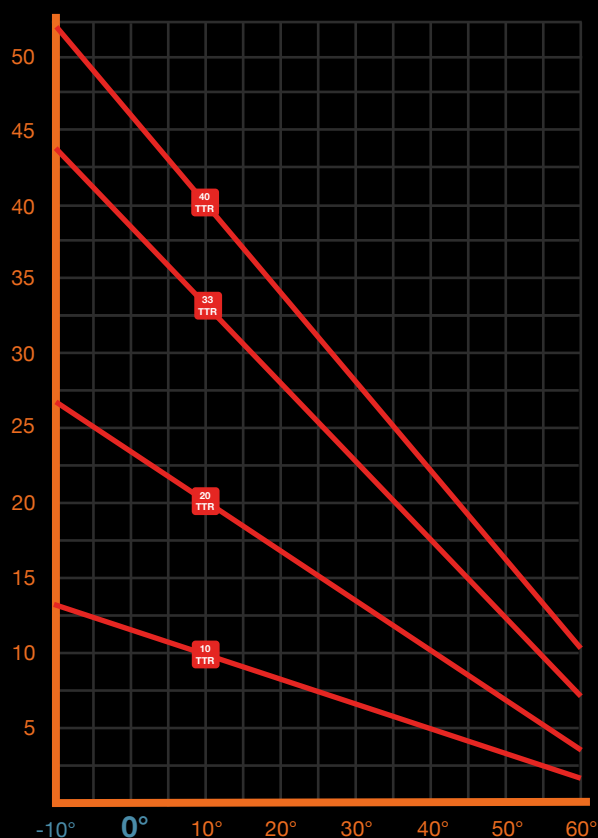
Temperature (°C) / Loading (W/m) diagram
